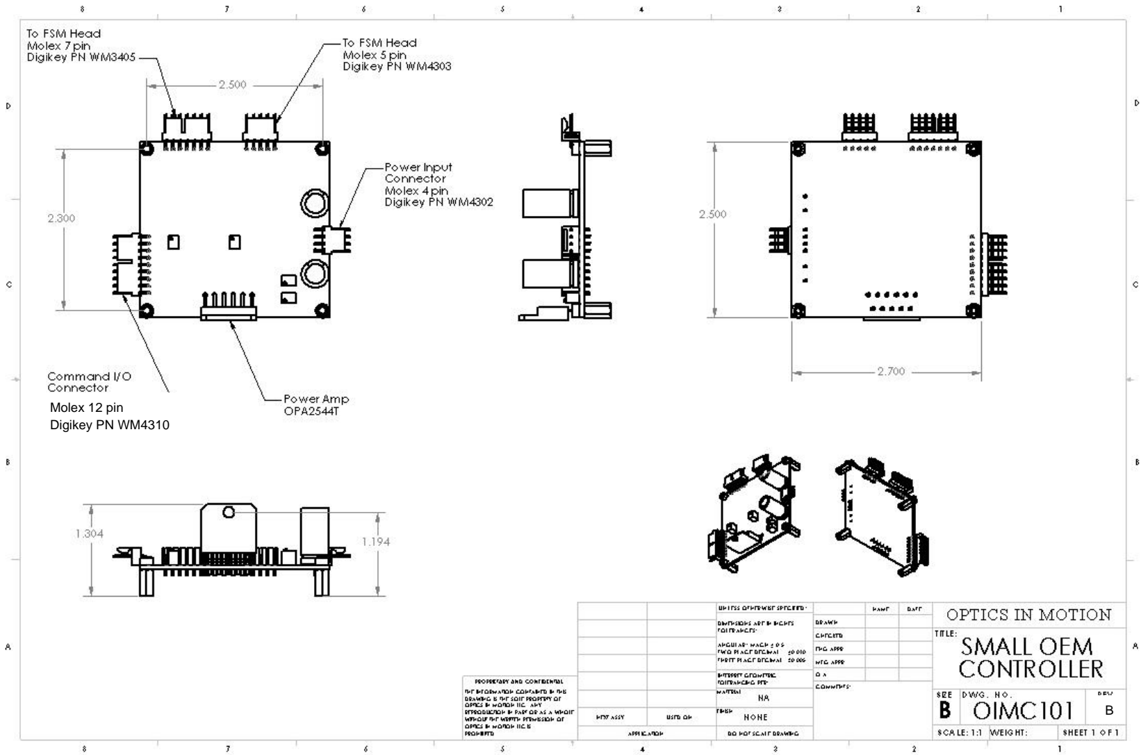
Figure 3: Small OEM Controller ICD
